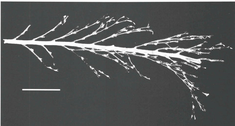
Fig. 1. Wimveria divergens (Naumov, 1960), lectotype colony. Scale bar 5 mm.
