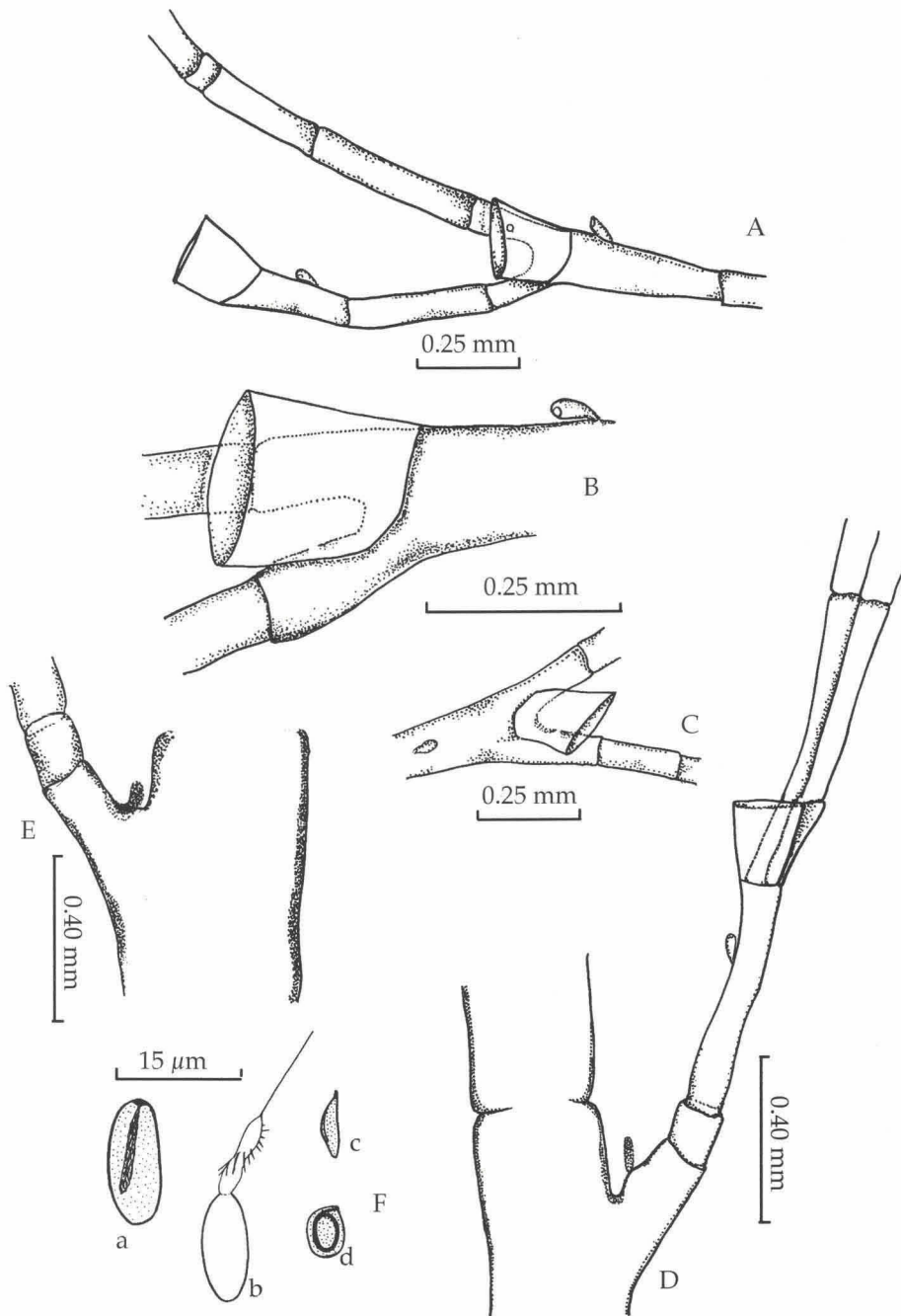
Fig. 3. Wimveria divergens , lectotype colony. A, forked hydrocladial internode; B, C, sections of hydrocladia with hydrothecae and intrathecal nemathothecae; D, E, sections of colony with cauline apophyses and nematophores; F, nematocysts: a, b, microbasic eurytele, undischarged (a) and discharged (b); c, microbasic mastigophore; d, desmoneme-like capsule.
