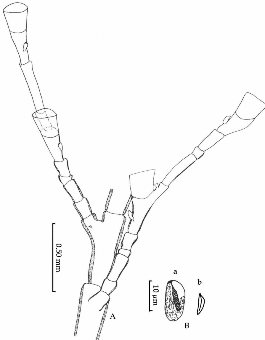
Fig. 8. Fragment of colony determined by O. Sheiko as Kirchenpaueriidae gen. sp. (North Kurile Islands, 48°N 155°E, 382-490 m); A, part of colony; B, nematocysts: microbasic eurytele (a) and microbasic mastigophore (b).
