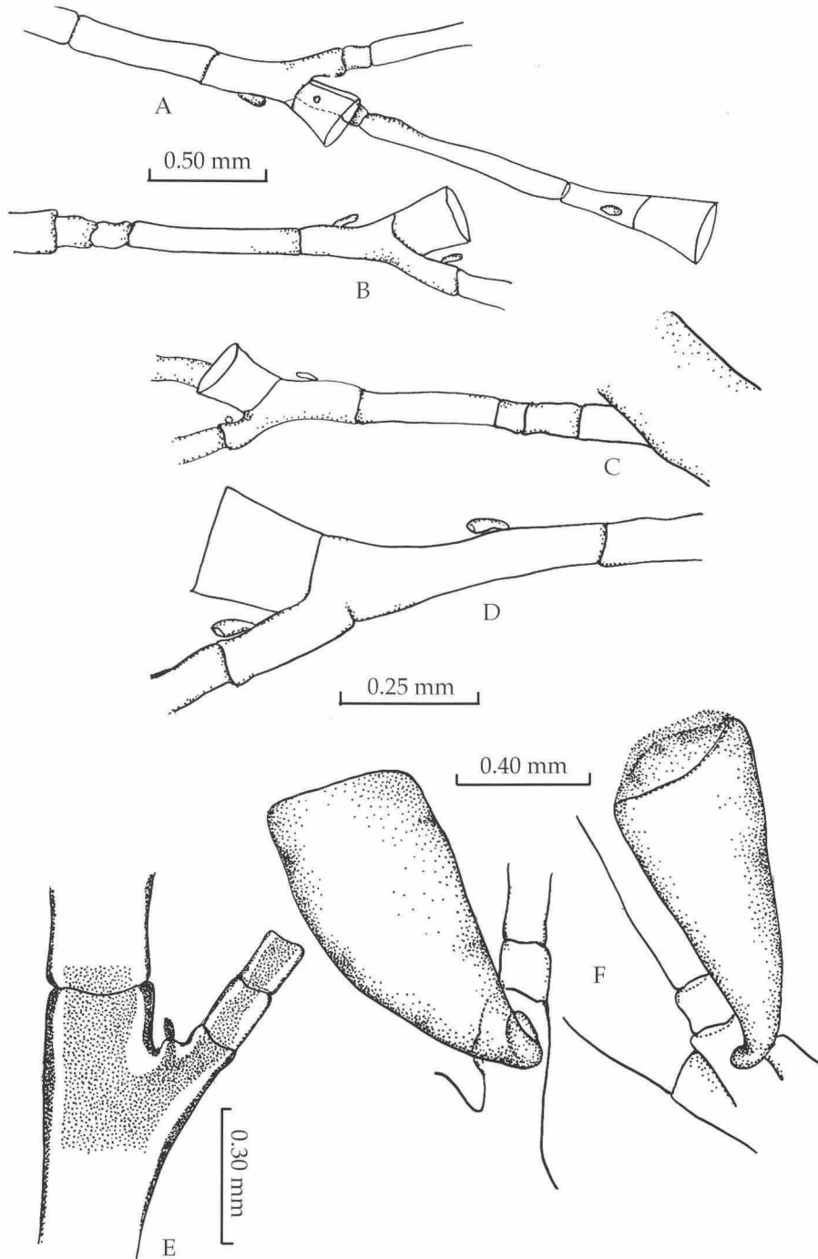
Fig. 5. Wimveria divergens . 'Odyssey', Iturup Island, 1100-1200 m. A-D, sections of hydrocladia with hydrothecae and nematothecae; E, cauline apophysis with 'mamelon' and nematophore; F, gonothecae.
